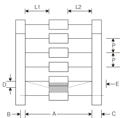
Taping Details
